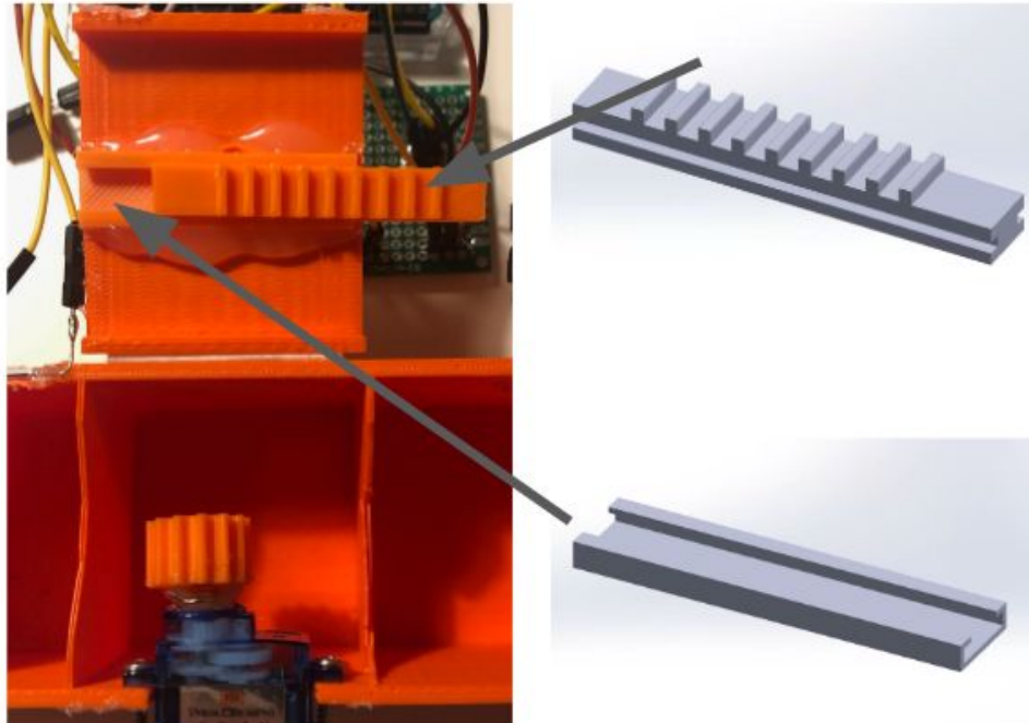
Figure 8: Locking Mechanism
