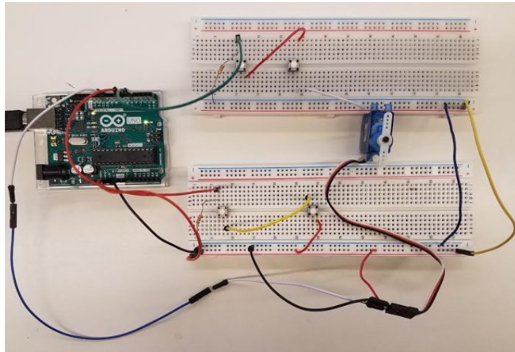
Figure 2: Locking Circuit
